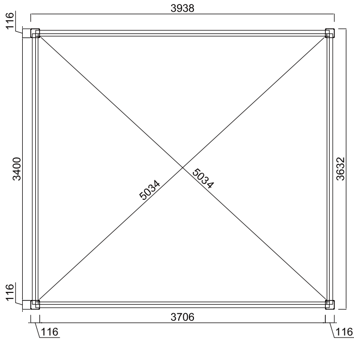
Base Plate Layout Plan
